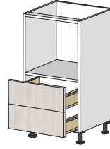
Base Oven 2 Drawer
